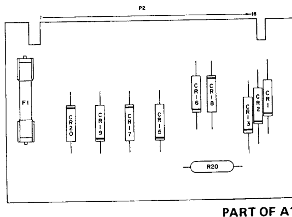
FIG. 6-2 COMPONENT LOCATION, PRINTED CIRCUIT BOARD (A1).
