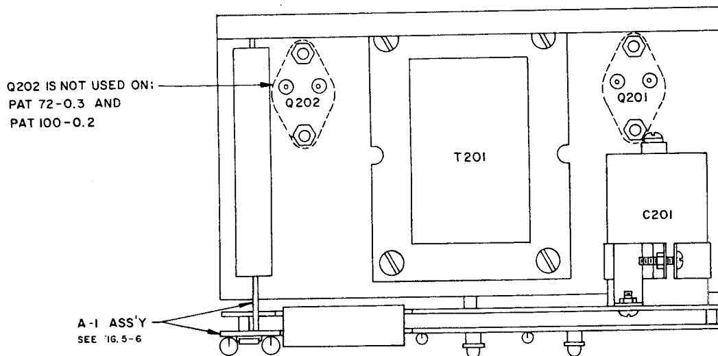
FIG. 6-1 COMPONENT LOCATION, MAIN CHASSIS ASSEMBLY (A2).
