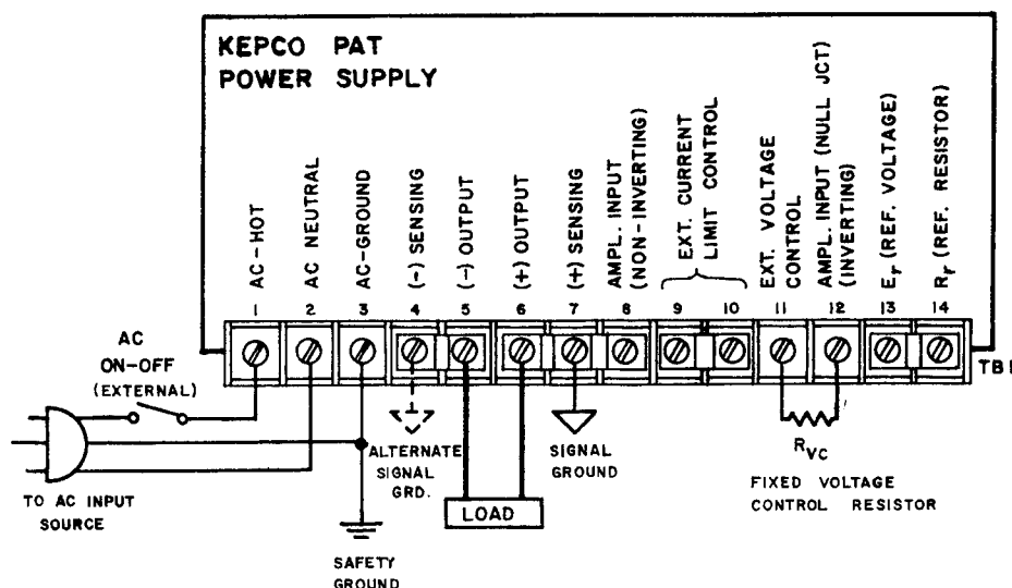
FIG. 3-1 CONNECTIONS FOR FIXED OUTPUT OPERATION.
